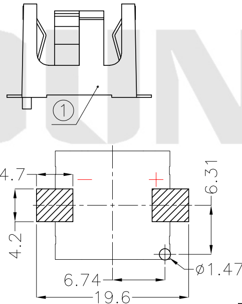
PCB Layout Diagram Top View
