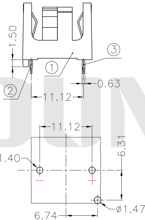
PCB Layout Diagram Top View
